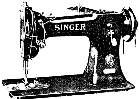
Fig. 2. Oiling Points at Front of Machine
