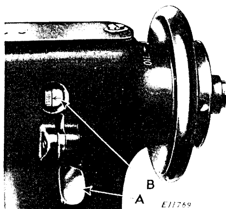
Fig. 17. Stitch Regulator
