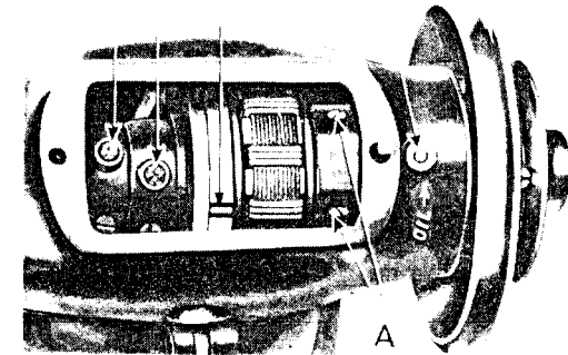
Fig. 4. Oiling Points in Arm of Machine
