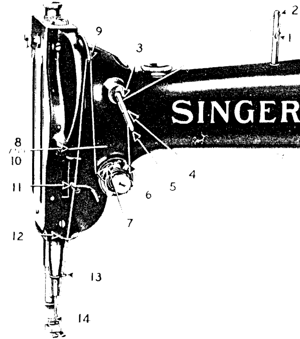
Fig. 13. Upper Threading
