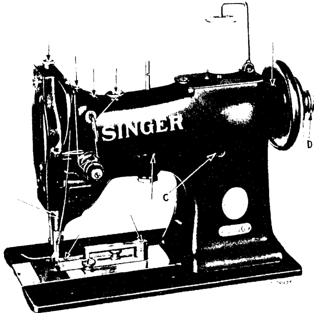
Fig. 2. Oiling Points at Front of Machine
