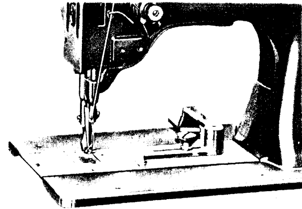
Guide 224697 Swung Out of Operation
