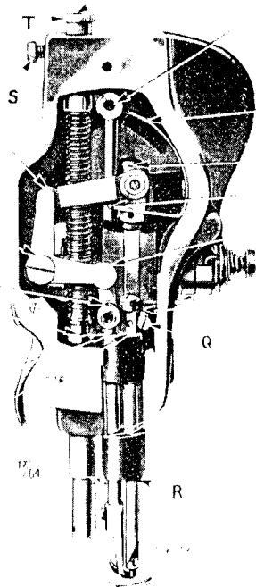
Fig. 6. Face Plate Removed for Oiling
