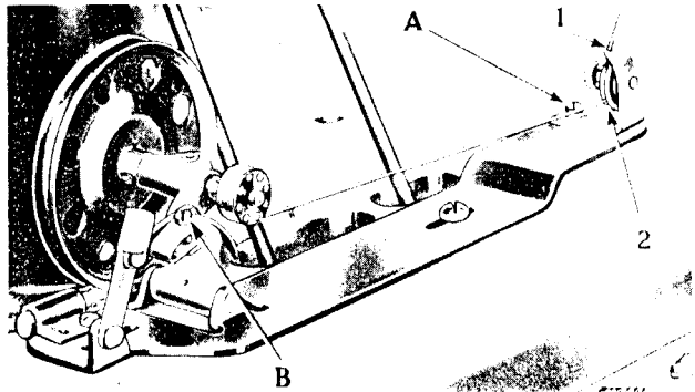
Fig. 10. Winding the Bobbin
