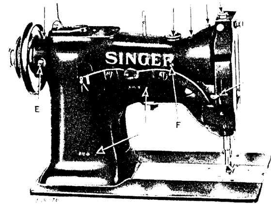
Fig. 5. Oiling Points and Adjustments at Rear of Machine
