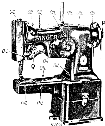
Fig. 4. Front View of Machine, Showing Oiling Points Also Adjustments on the Machine
